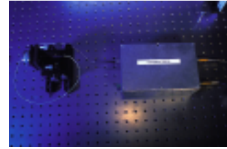
Coupler device separates photons' pairs and turn them toward two fibre- optics.
